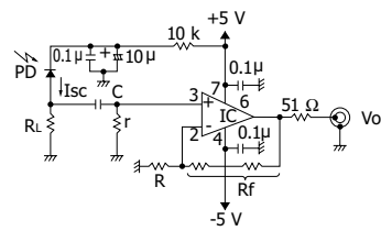
[Figure 16] AC photodetector circuit (1)
