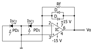
[Figure 10] Light balance detection circuit
