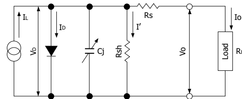
[Figure 3] Photodiode equivalent circuit
