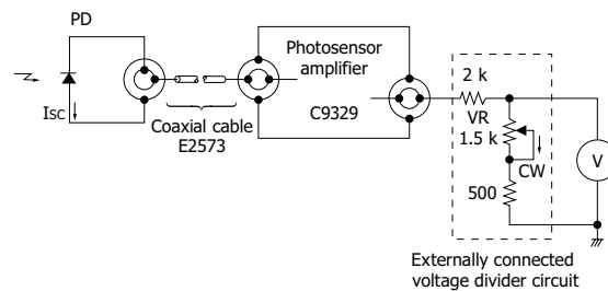
[Figure 8] Basic illuminometer (1)
